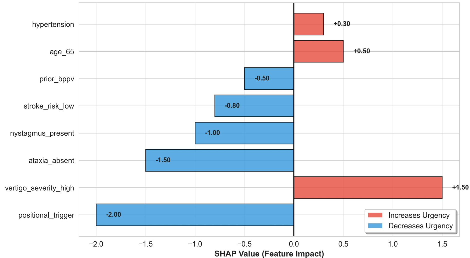
SHAP Feature Importance for DRAS-5 Classification
