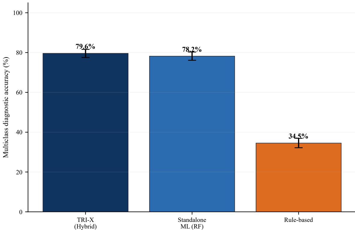
Diagnostic accuracy on held-out synthetic test set (n=1500)
