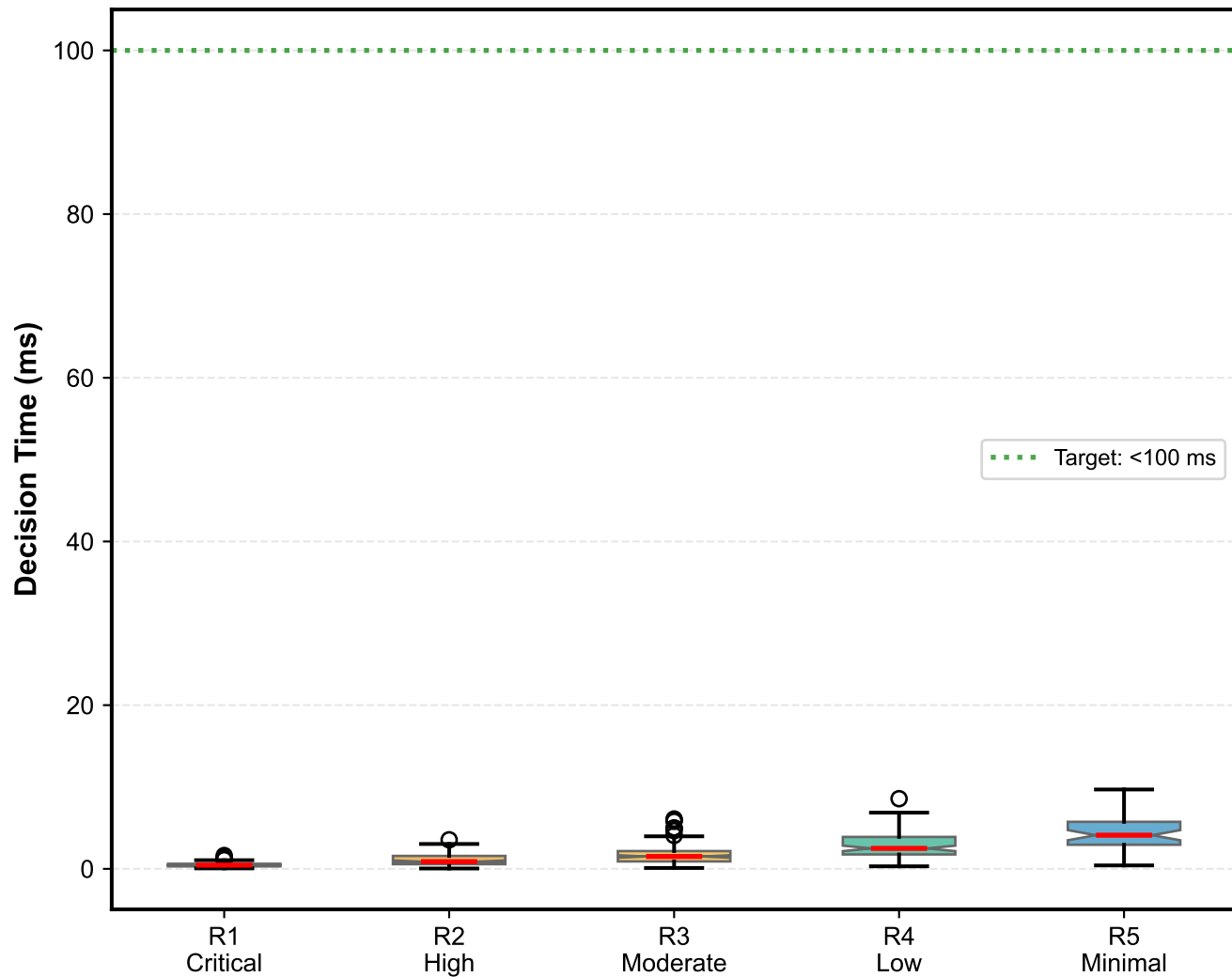
B. Decision Time by Risk Tier
