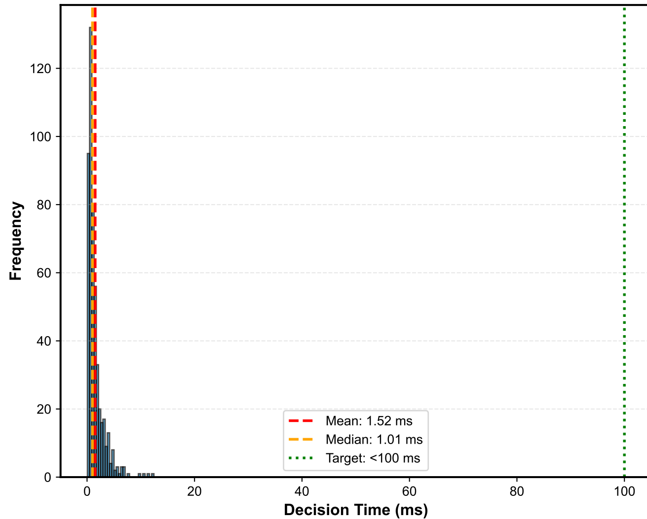
A. Decision Time Distribution (n=500)
