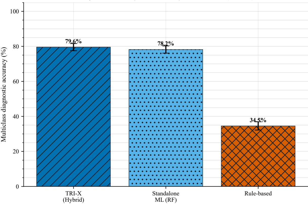
Diagnostic accuracy on held-out synthetic test set (n=1500)
