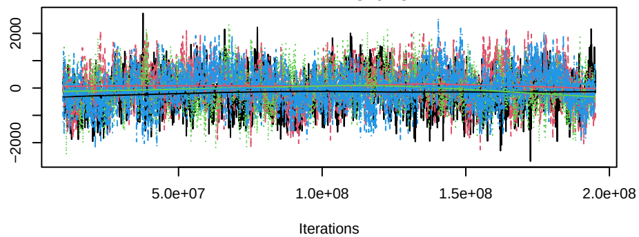
Trace of mutual
