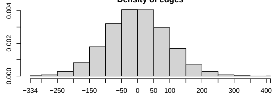
Density of edges
