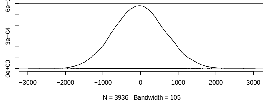
Density of mutual
