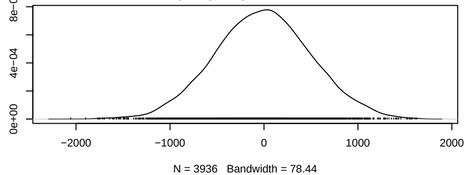
Density of gwdsp.OTP.fixed.0.025
