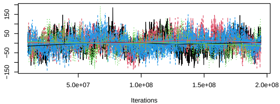
Trace of gwideg.fixed.0.025
