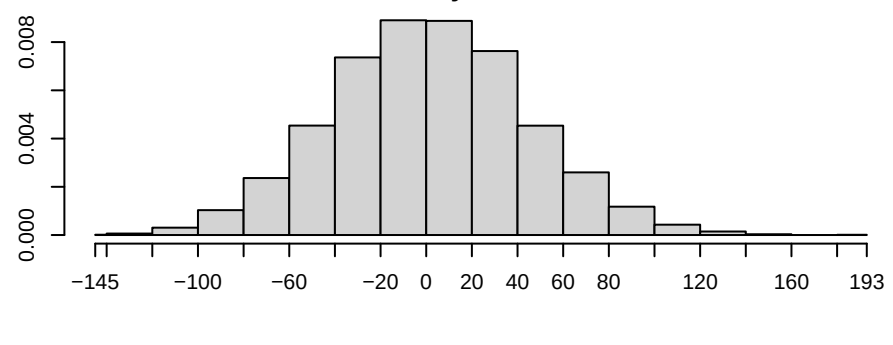
Density of gwideg.fixed.0.025
