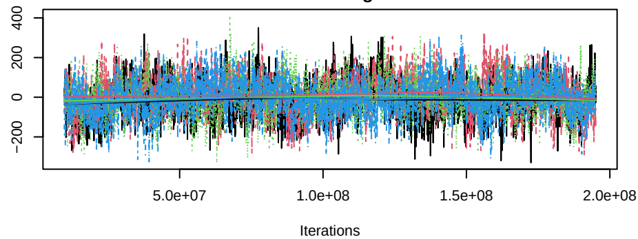
Trace of absdiff.regulatory_quality
