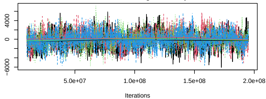
Trace of nodecov.log_total_imports
