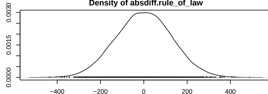
Density of absdiff.rule_of_law
