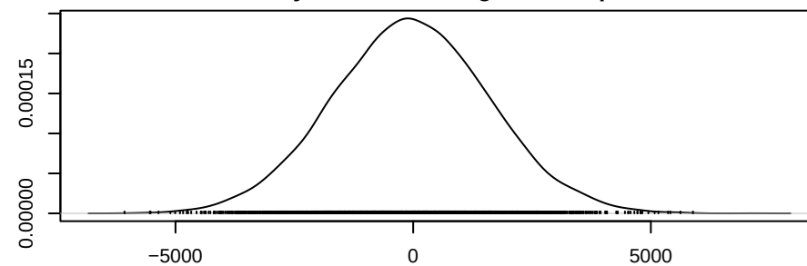
Density of nodecov.log_total_imports
