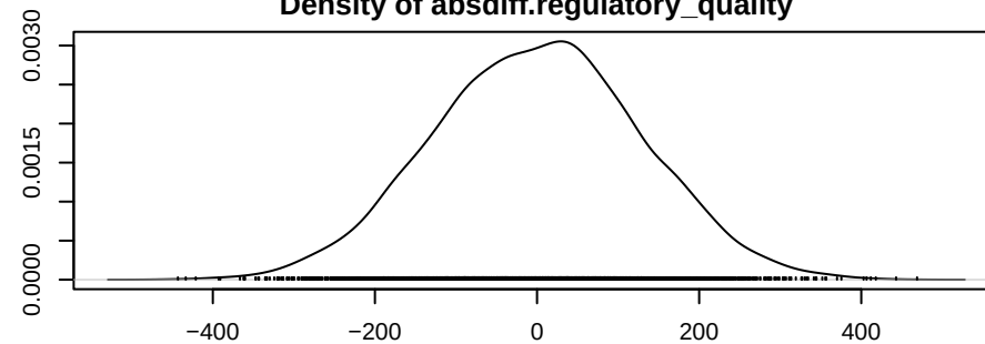
Density of absdiff.regulatory_quality
