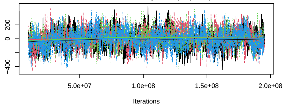
Trace of absdiff.rule_of_law
