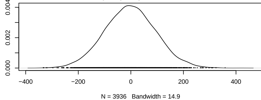
Density of gwesp.OTP.fixed.0.025
