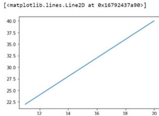
Figure 2.44: Line plot
