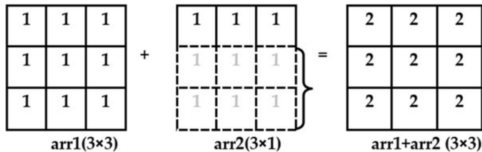
Figure 2.12: NumPy broadcasting
