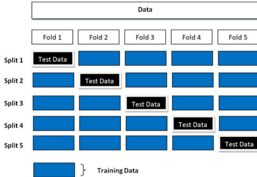
Figure 3.21: K-fold cross-validation
