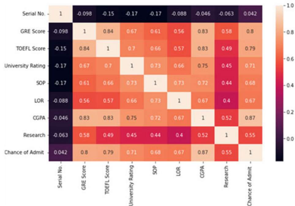
Figure 2.59: Heatmap
