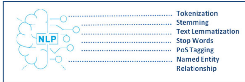
Figure 6.4: NLP pipeline
