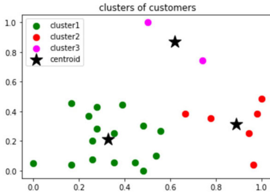
Figure 3.44: Cluster visualization
