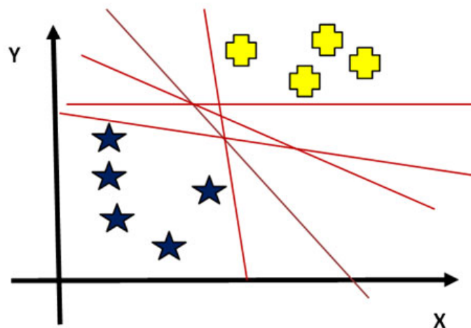
Figure 3.17: SVM classification
