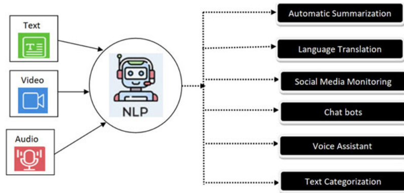
Figure 6.1: NLP applications
