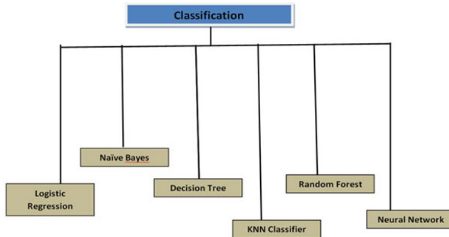
Figure 3.13: Classification algorithms
