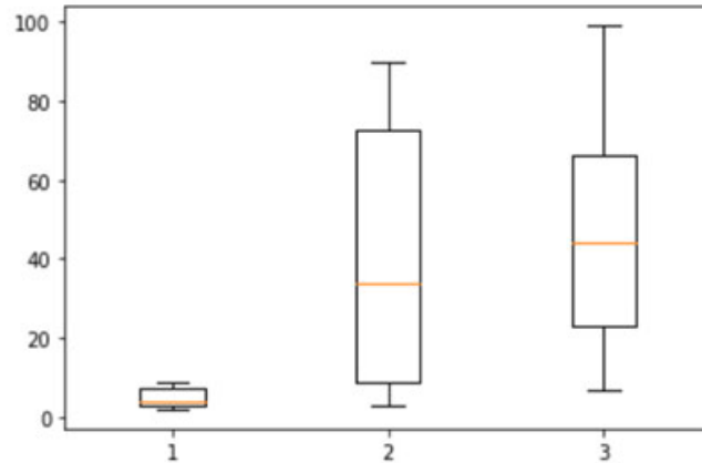
Figure 2.53: Box plot
