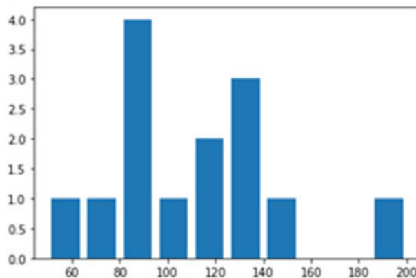
Figure 2.51: Plotting histogram
