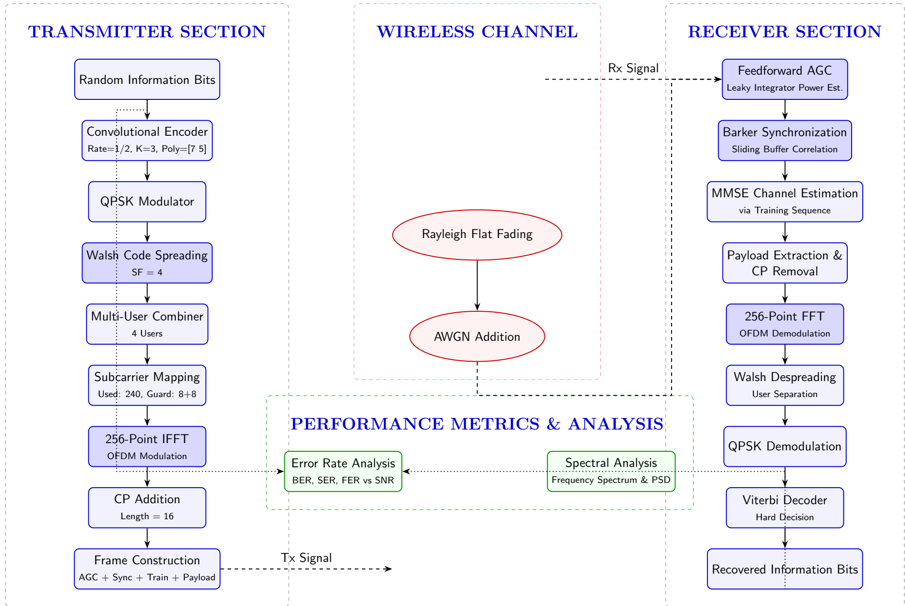
1 Figure 1: Complete System Architecture of the Proposed MC-CDMA Transceiver
