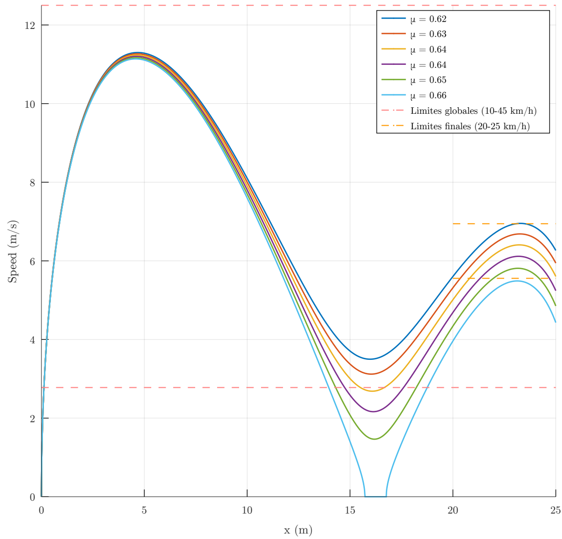
Speed vs Position for Different Friction Coefficients
