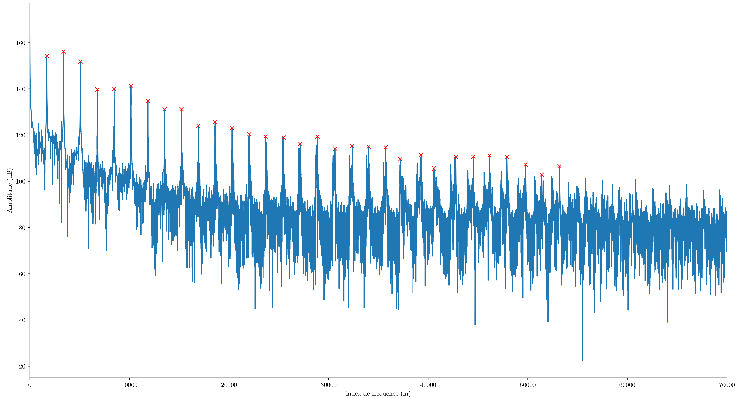
Harmonics identification
