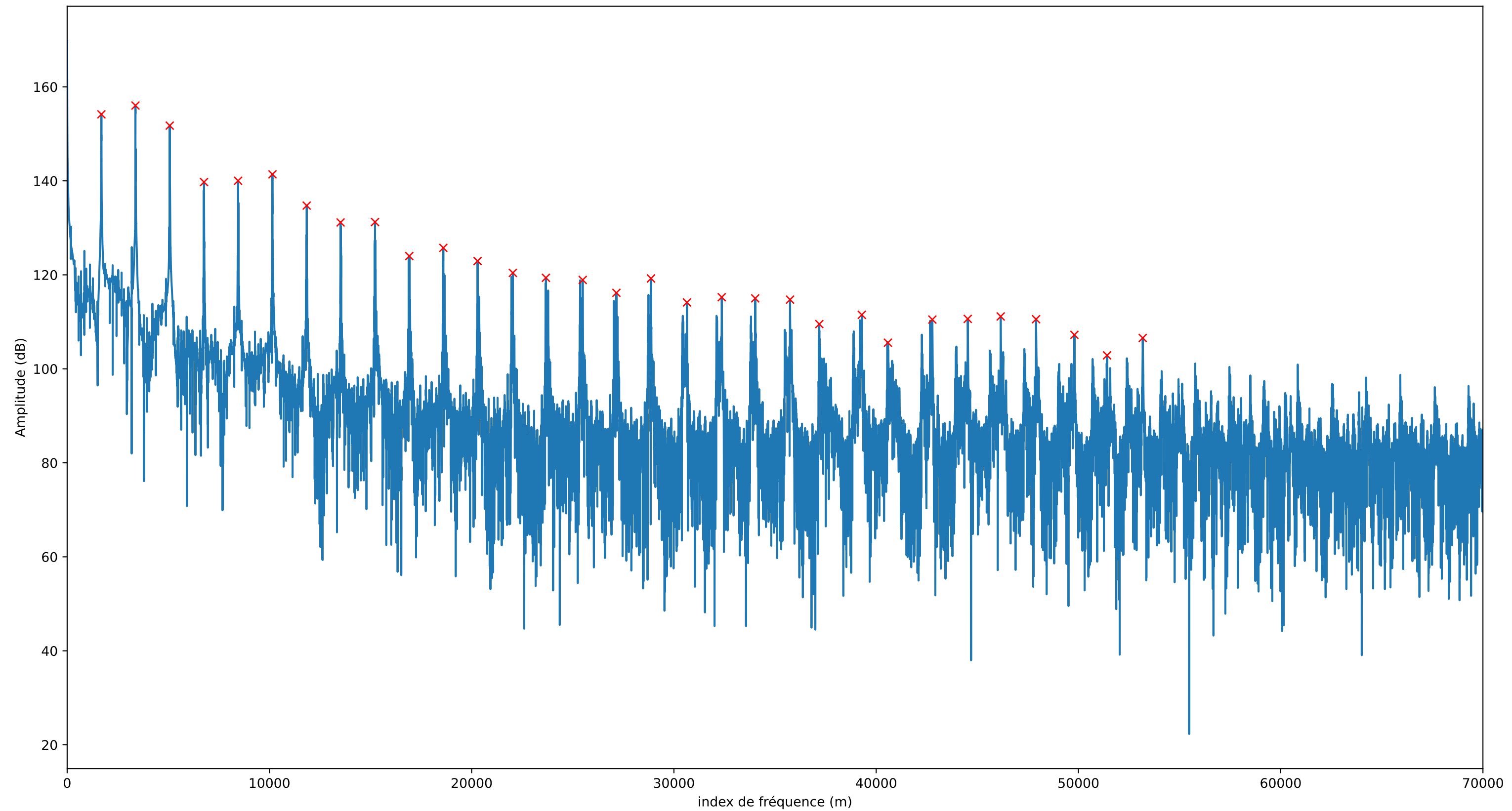
Harmonics identification
