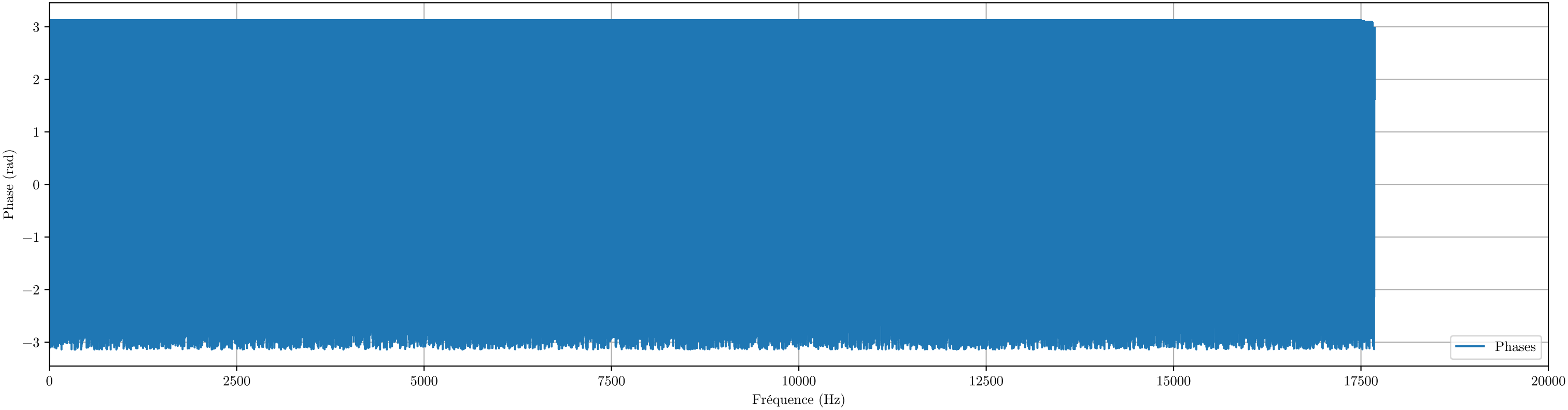
Spectre de phases de synthesized note_guitare_lad
