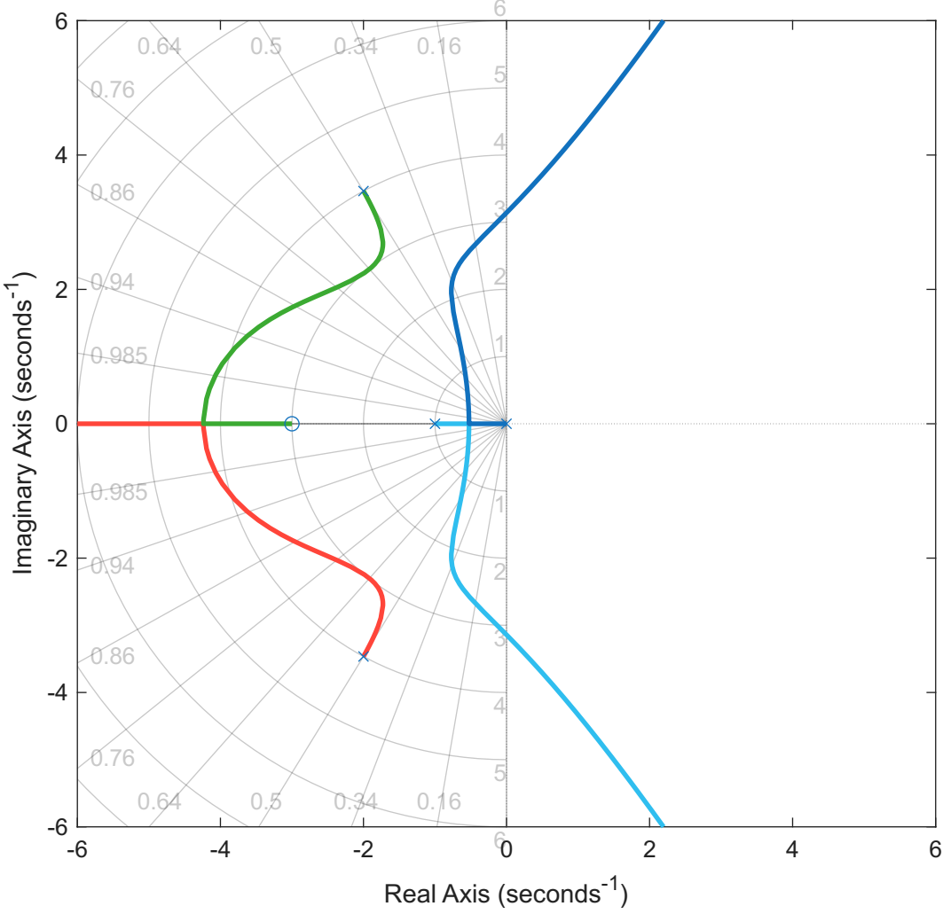
Root Locus
