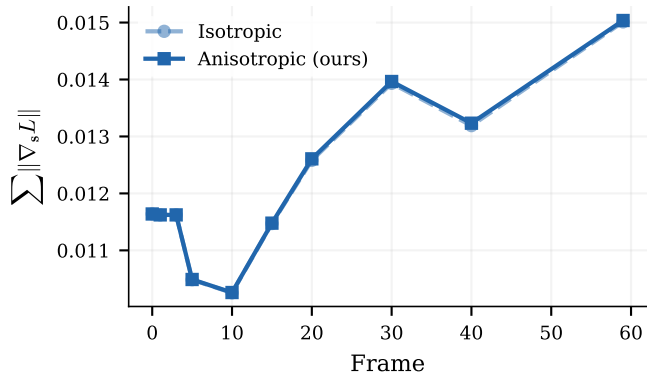
(a) Scale gradient \nabla_s L
