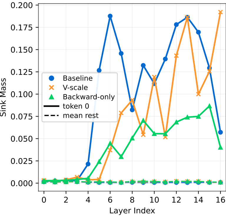
Attention Sink Mass (0.3B)
