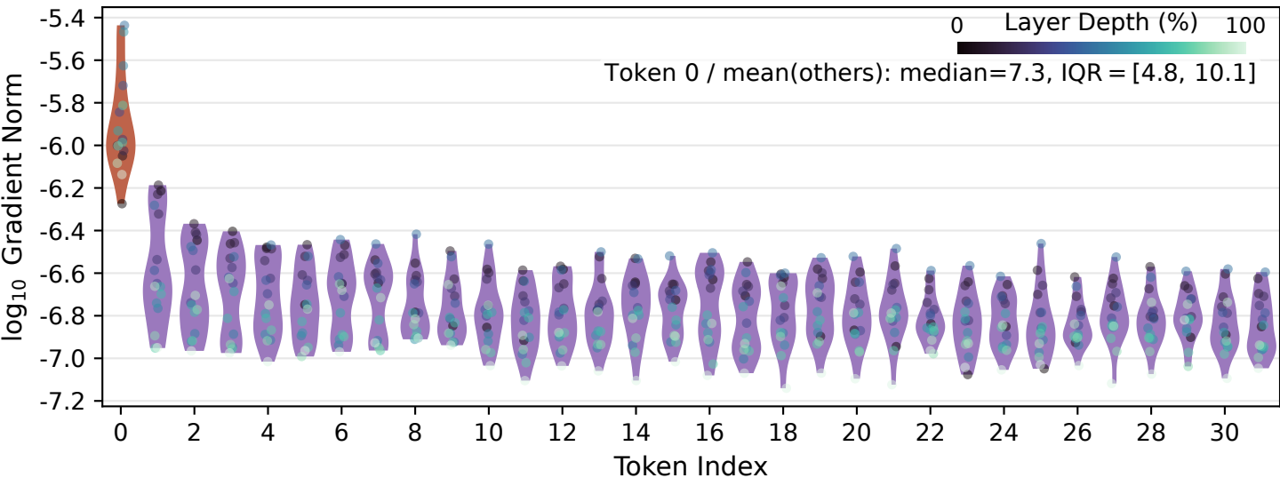
Gradient Distribution at the Attention Input (after RMSNorm) of 0.1B V-scale
