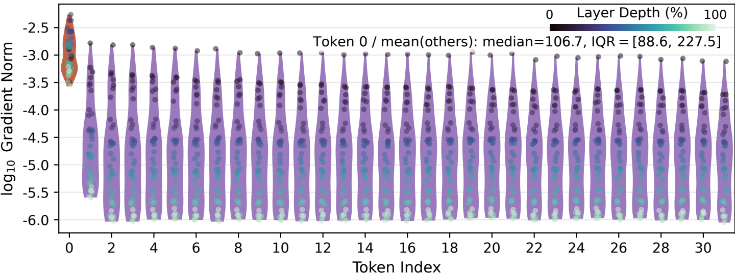
Gradient Distribution at the Attention Input (after RMSNorm) of Qwen3-8B
