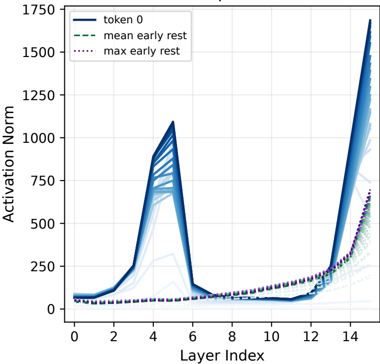
MLP Output Norm
