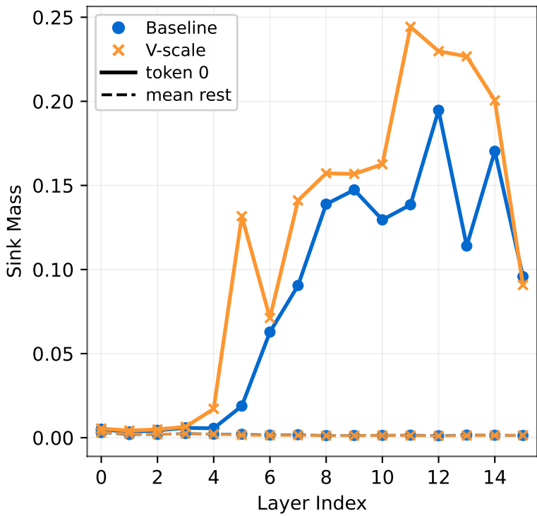
Attention Sink Mass (0.1B)
