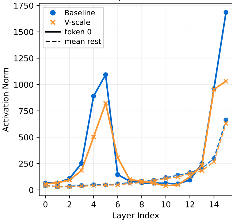
MLP Output Norm (0.3B)
