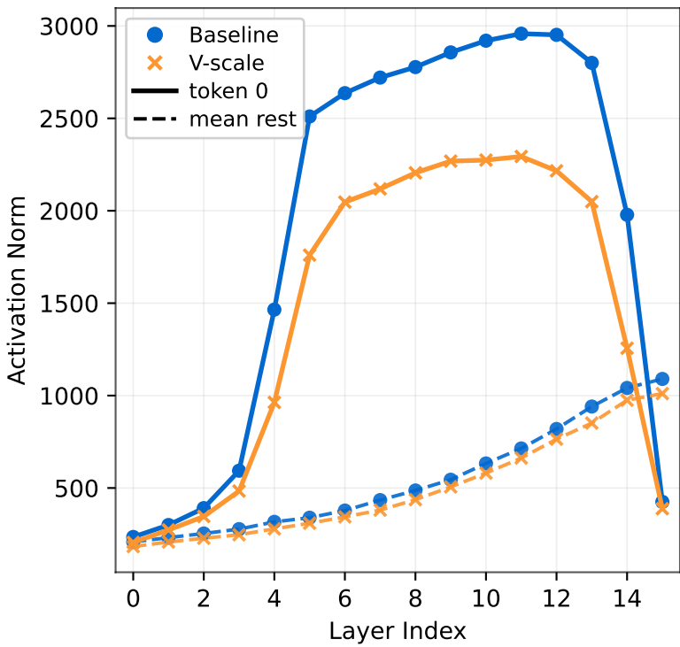
Residual-Stream Output Norm (0.3B)
