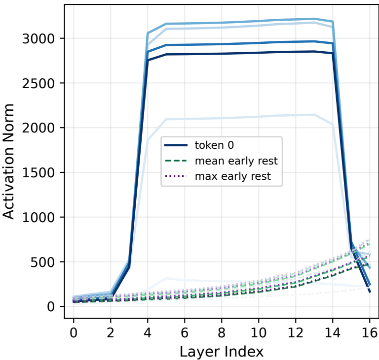
Residual-Stream Output Norm
