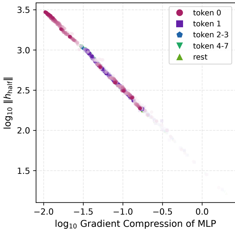
Gradient Compression vs. Activation
