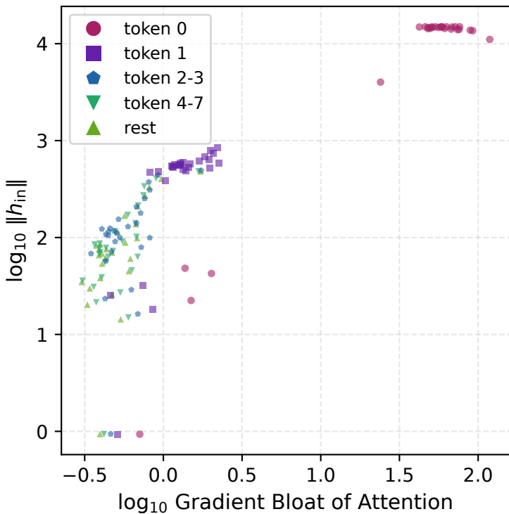
Gradient Bloat vs. Activation
