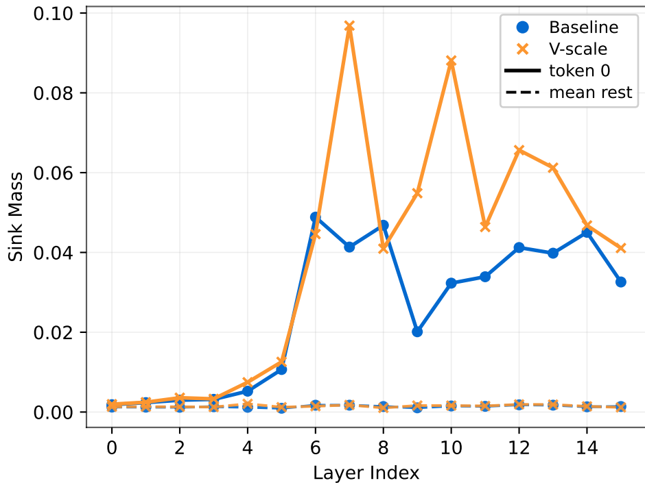
Attention Sink Mass (0.3B)
