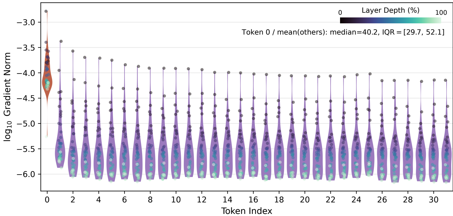
Gradient Distribution at the Attention Input (after RMSNorm) of GLM-4-9B
