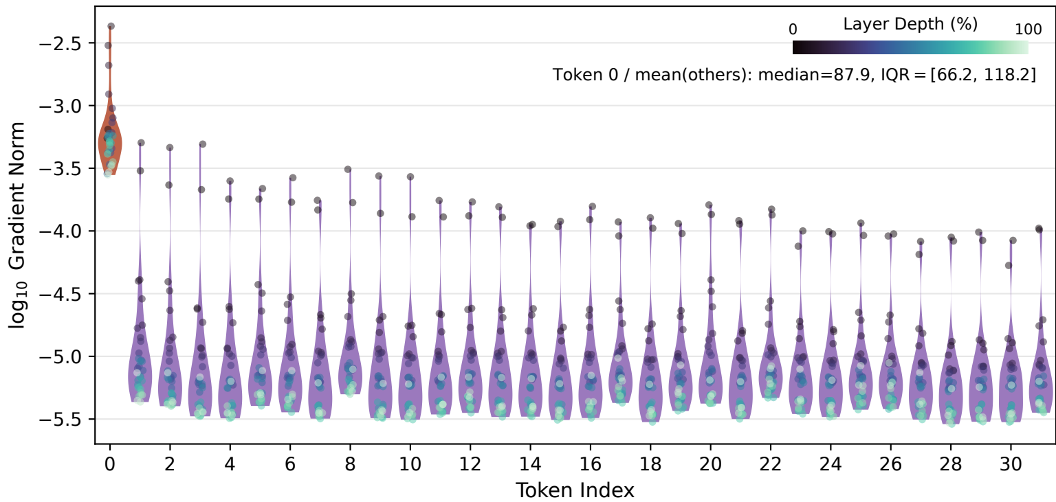
Gradient Distribution at the Attention Input (after RMSNorm) of Llama-3.1-8B
