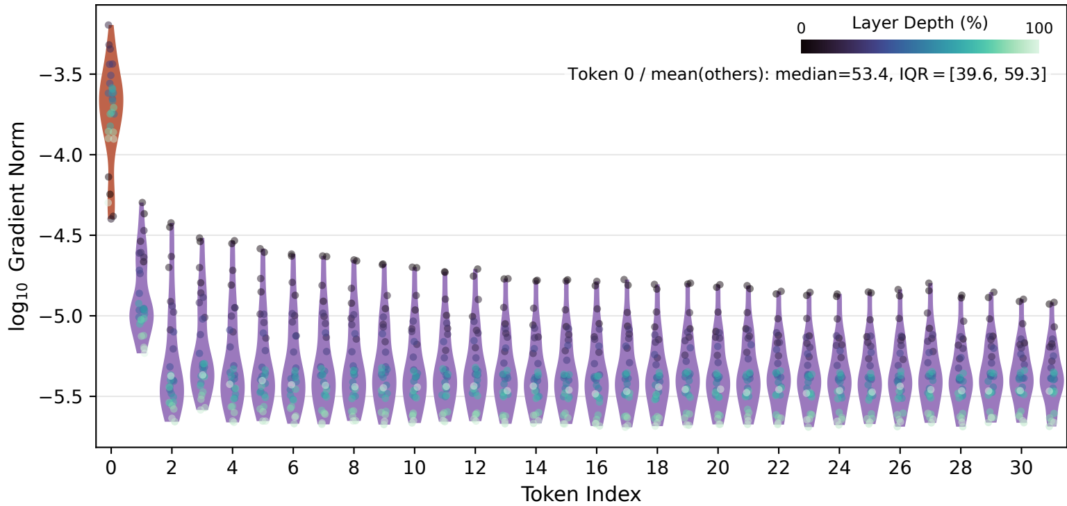
Gradient Distribution at the Attention Input (after RMSNorm) of Qwen2.5-7B
