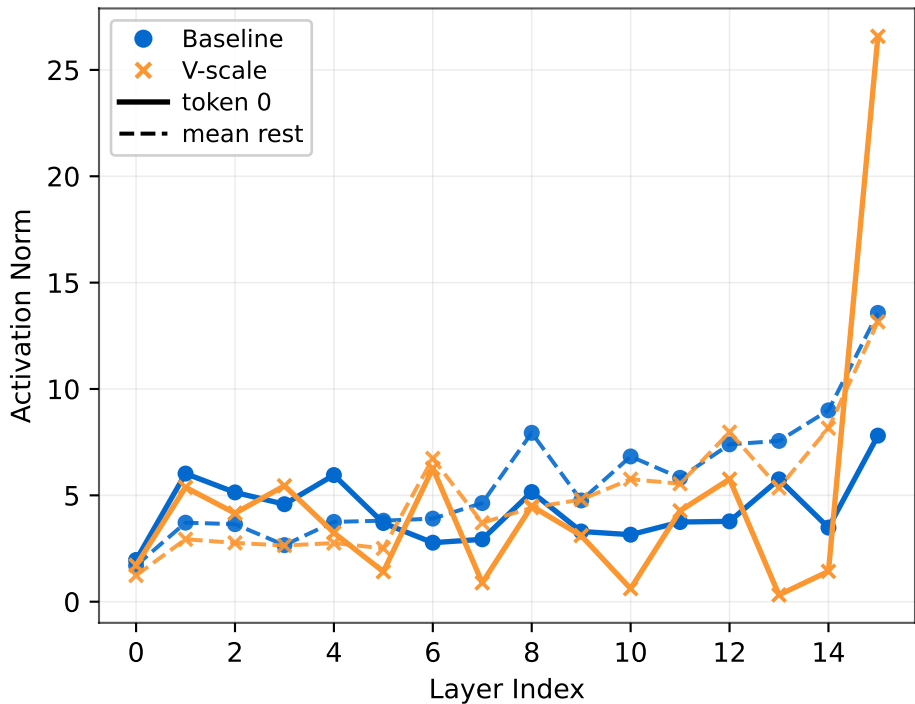
Attention Output Norm (0.1B)
