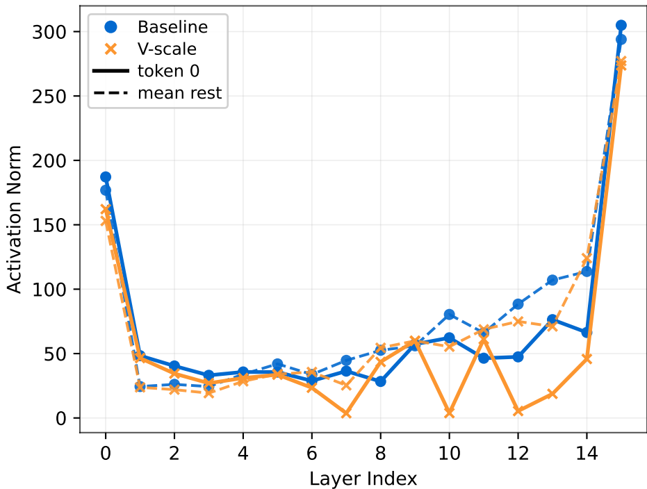
Attention Output Norm (0.3B)
