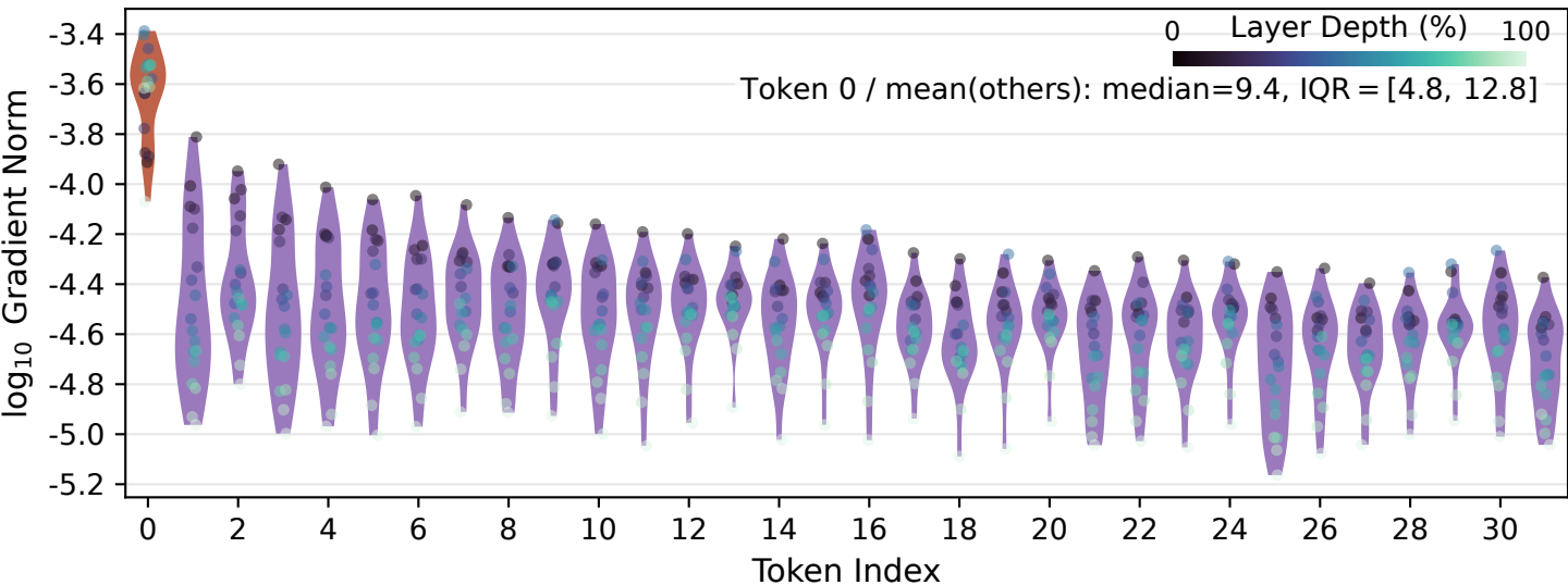
Gradient Distribution at the Attention Input (after RMSNorm) of 1B Baseline
