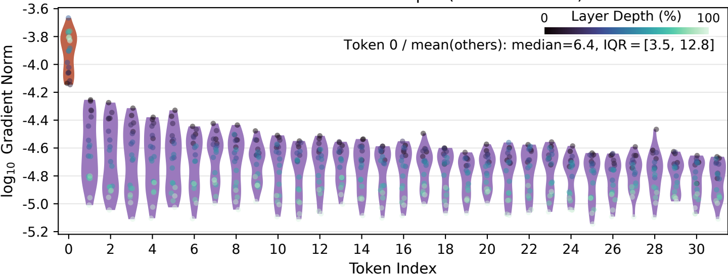
Gradient Distribution at the Attention Input (after RMSNorm) of 1B V-scale
