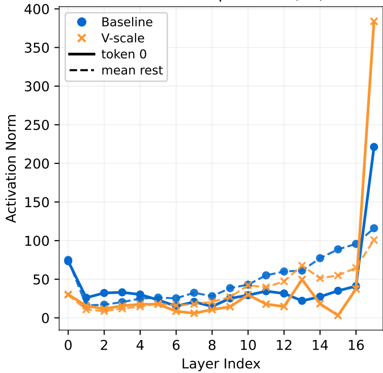
Attention Output Norm (1B)
