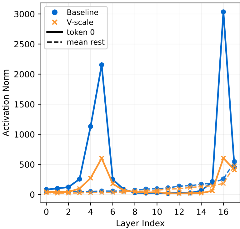
MLP Output Norm (1B)
