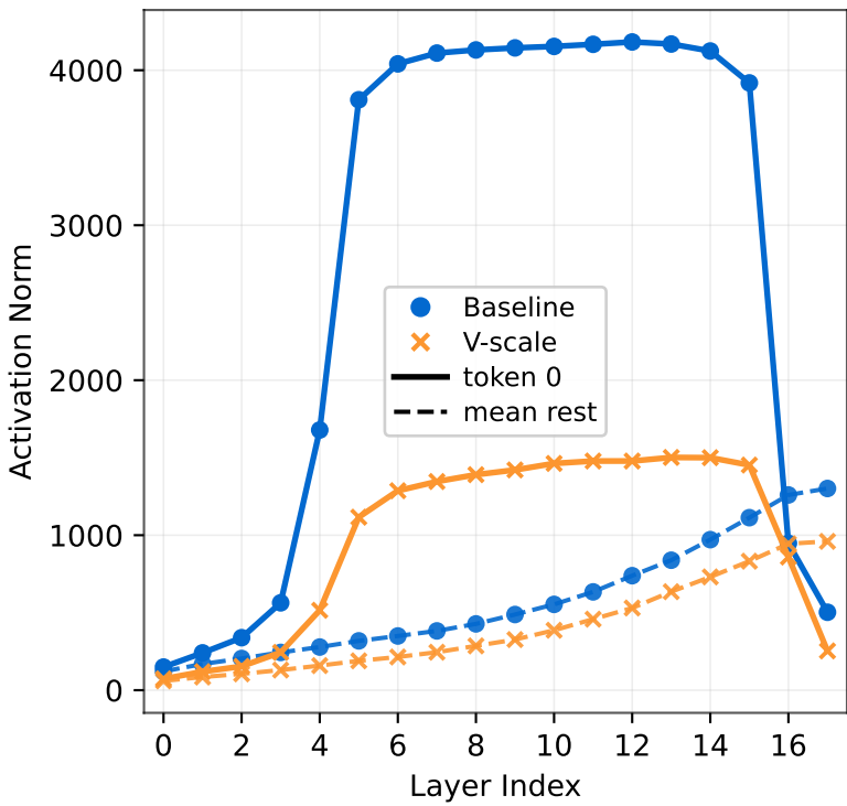
Residual-Stream Output Norm (1B)
