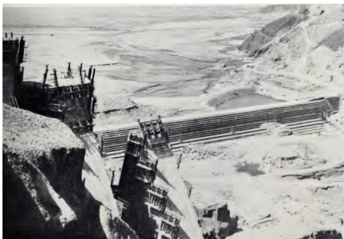
The Sefid Roud dam under construction.
