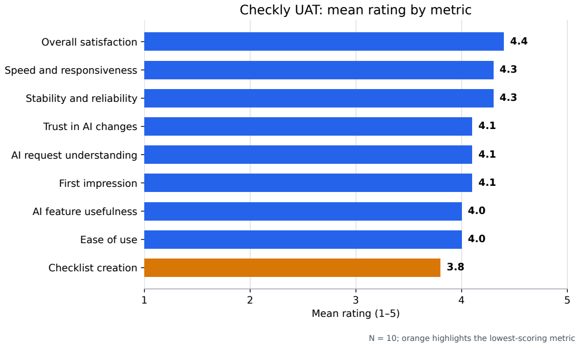
Figure 1: Mean rating for each UAT metric on the five-point scale.
