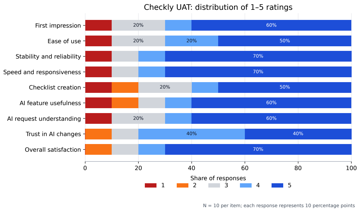
Figure 2: Distribution of the 1–5 ratings for each UAT metric.
