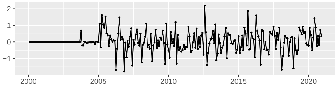
Residuals from ARIMA(0,1,3)(0,0,1)[12]
