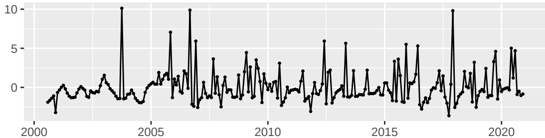
Residuals from Regression with ARIMA(1,0,1) errors
