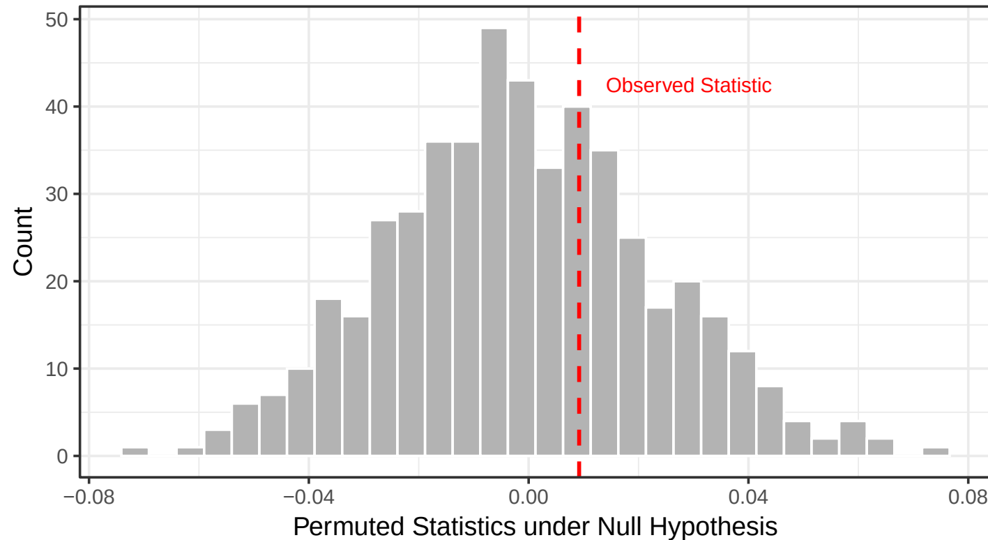
Linkage: PKC \rightarrow PKA
