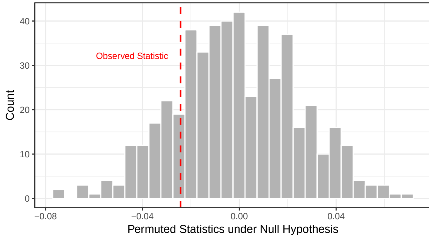
Linkage: (PIP2, PLCg) \rightarrow PKC
