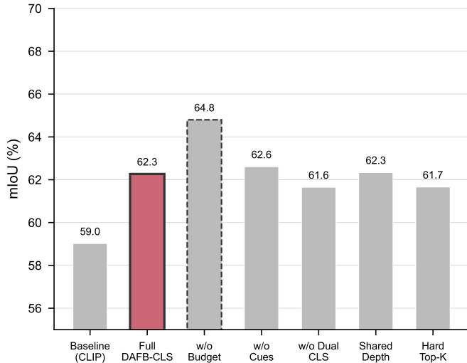
Ablation: OpenCLIP ViT-B/16 + VOC
