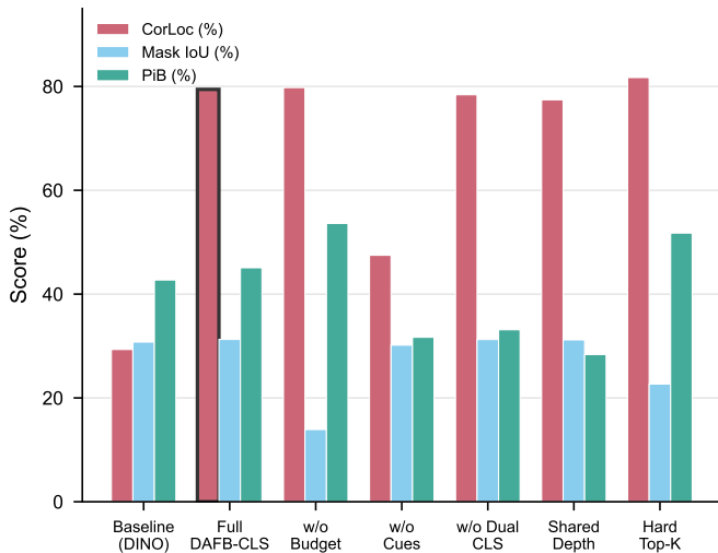
Ablation: DINO ViT-S/16 + VOC
