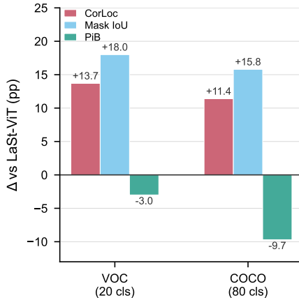
Improvement Deltas
