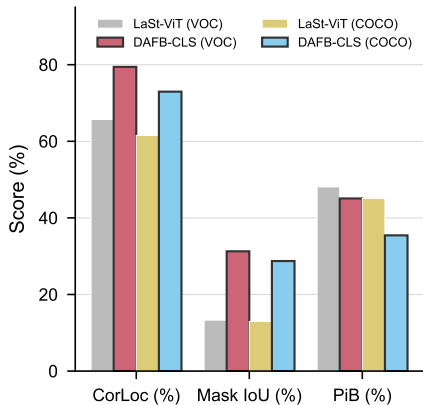
Absolute Scores
