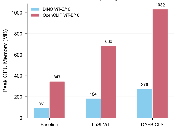
Memory Usage
