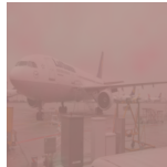
FG mask
