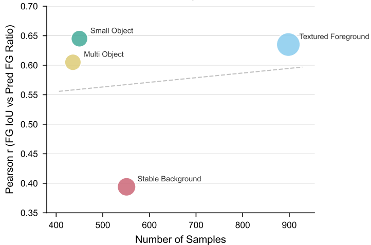
Prediction-Quality Correlation
