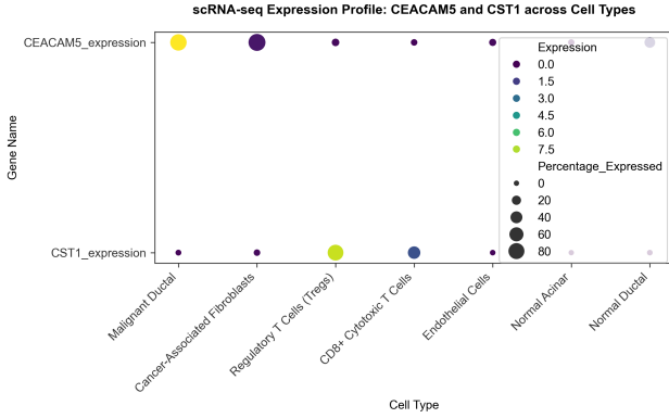
Fig. 9: Illustrative scRNA-seq dotplot showing cell-type specific expression of CEACAM5 and CST1 (illustrative data only).
