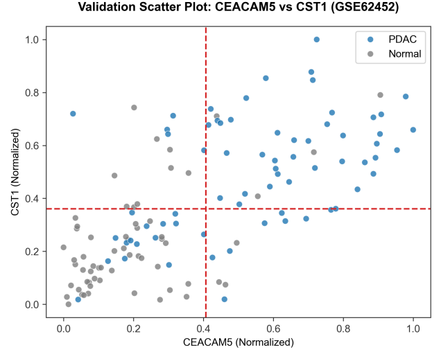
Fig. 8: CEACAM5 vs CST1 expression in GSE62452 validation cohort demonstrating transferability.
