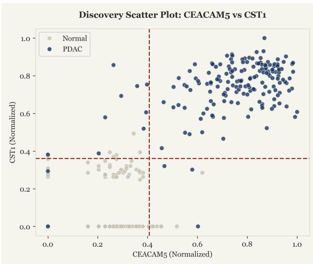
Fig. 7: CEACAM5 vs CST1 rescaled expression in the discovery cohort showing the decision quadrants.
