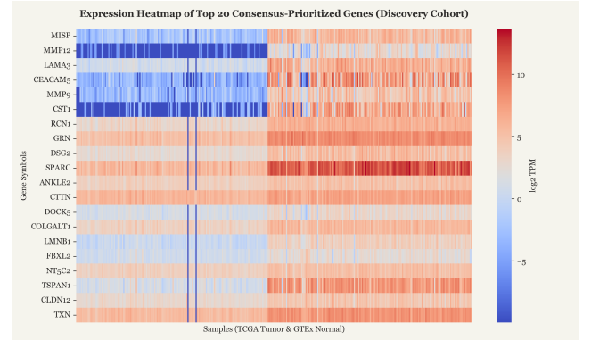
Fig. 6: Expression heatmap of top consensus-prioritized genes in the discovery cohort.
