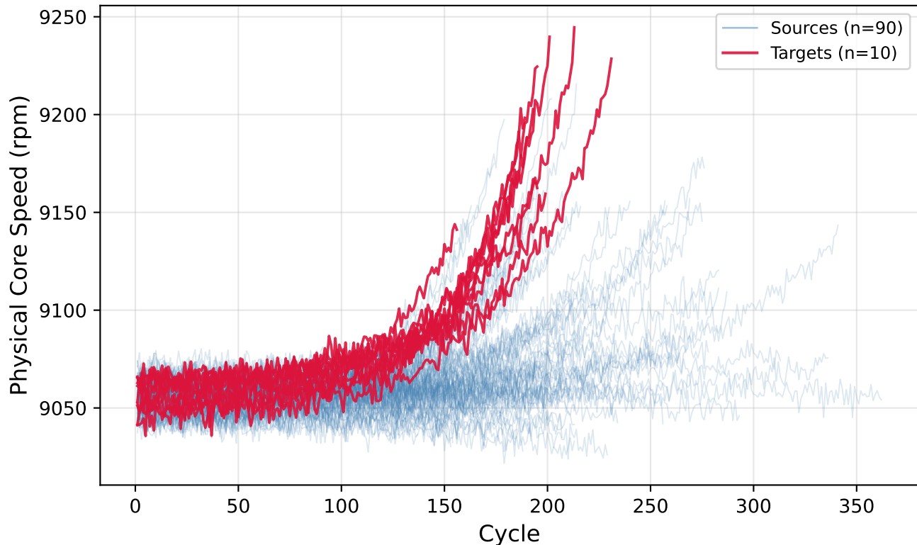
Physical core speed trajectories (red: target machines for evaluation, n=10)
