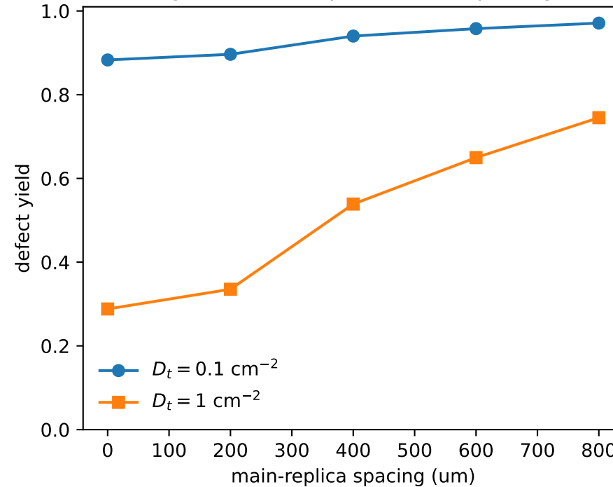
Fig. 19: W2W representative pairing
