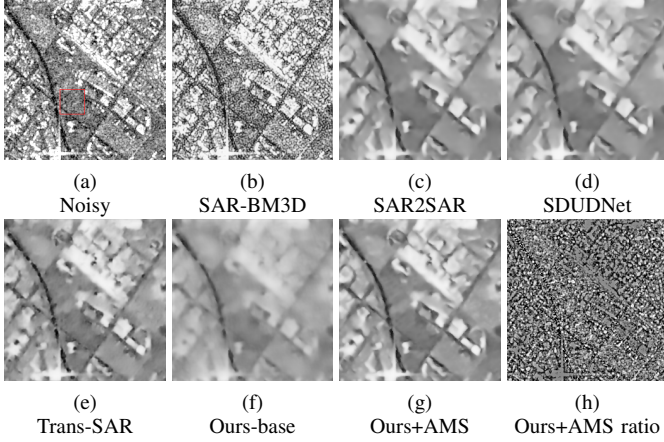
Fig. 5. Qualitative comparison on one real-SAR scene. Ours-base is the pre-adaptation model. Original renderings, including the red box for visual inspection in (a), are retained. The Ours+AMS ratio in (h) is interpreted separately from restored images. No clean reference is shown.
