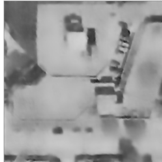
(c) LEE
