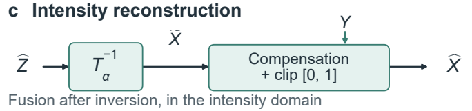
Fig. 1. (a) Encoder–decoder overview; tensor labels give spatial size \times channels. Gray marks inherited operators, and colors mark additions. Six FDR blocks have independent parameters. (b) Decoder order: skips concatenate encoder features before fusion; D_0 has no skip. GM denotes stage-specific guidance modulation using the resized shared map G . (c) Log predictions are inverted before intensity compensation with original Y and clipping.
