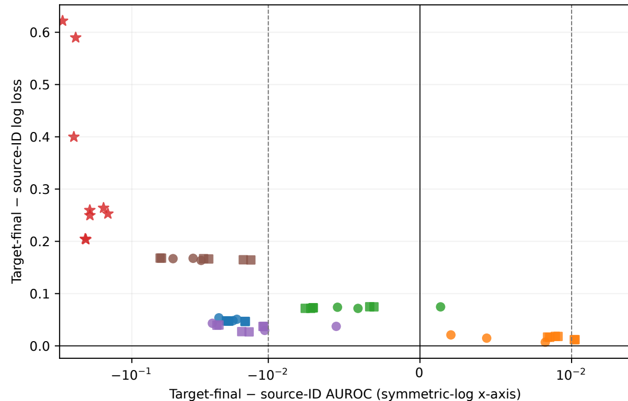
B. Log loss
